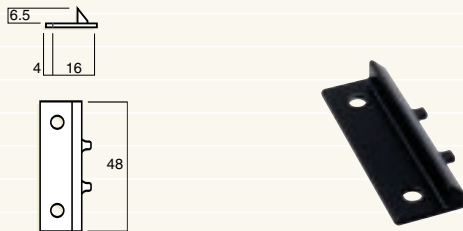
16 mm flat strike
