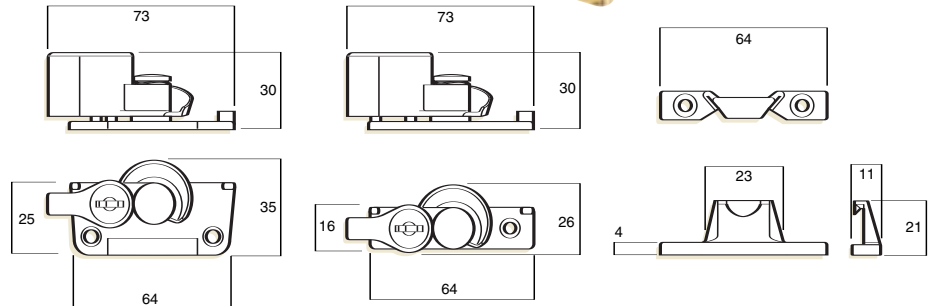
Wide base
