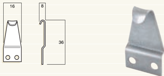
Alcan keeper
