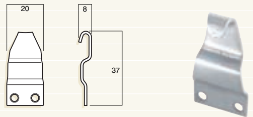
Comalco keeper
