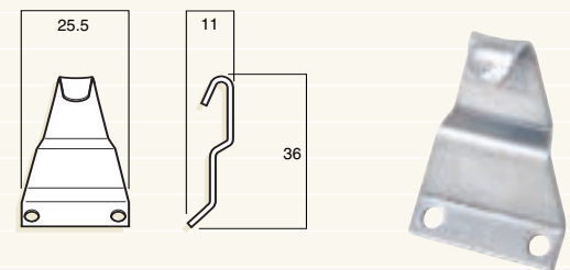
Altherm keeper
