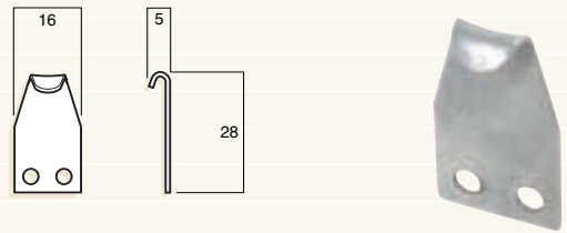
Wideline keeper
