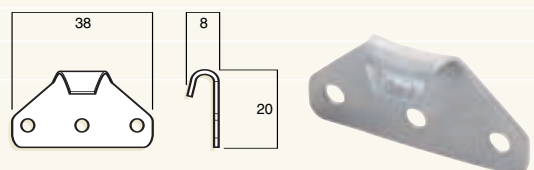
Altherm keeper
