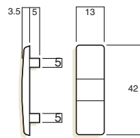
3.5 mm Nylon Strike
