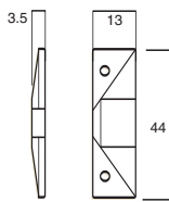
9.0 Nylon Strike
