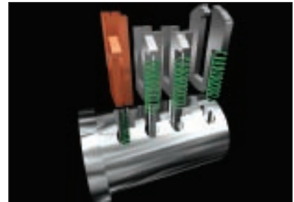
The patented CYL4™ cylinder has been designed to retain its wafers when the key is removed. This makes re-keying the CYL4™ cylinder quick and easy for retailers and locksmiths alike.
