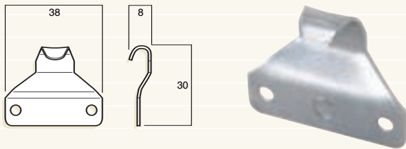
Modified Dowell keeper
