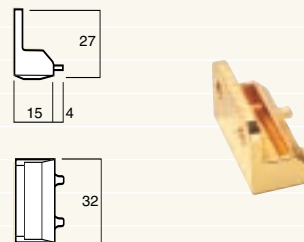
Timber frame strike
