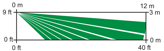
Side View Broad: 12 m x 12 m
